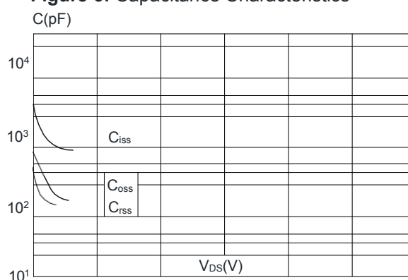
Figure 6: Capacitance Characteristics
