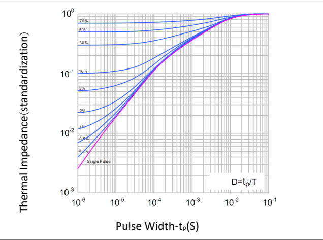
Figure 14 Transient thermal impedance VS Pulse Width
