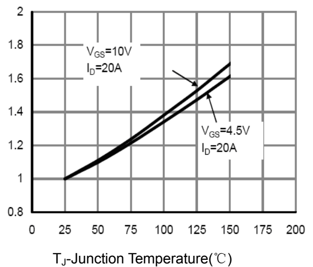
Figure 4 Rdson-Junction Temperature
