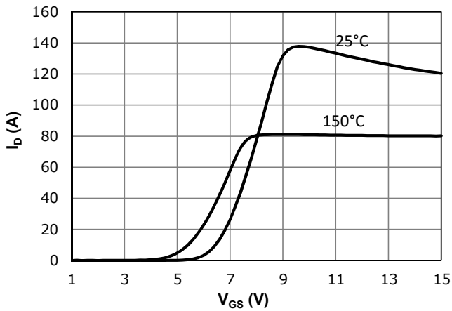
Fig 3: Transfer Characteristics
